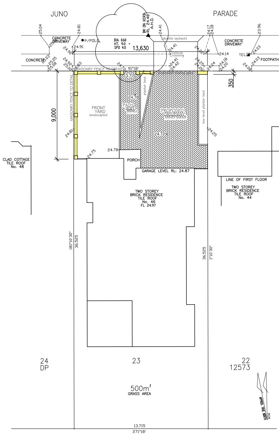
SITE / GROUND FLOOR PLAN SCALE 1 : 200
